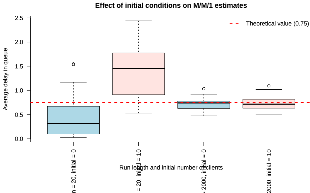
Figure 8: Distribution of the 25 average queue-delay estimates for each run length and initial condition. The dashed line marks the theoretical value W_Q = 0.75 .
