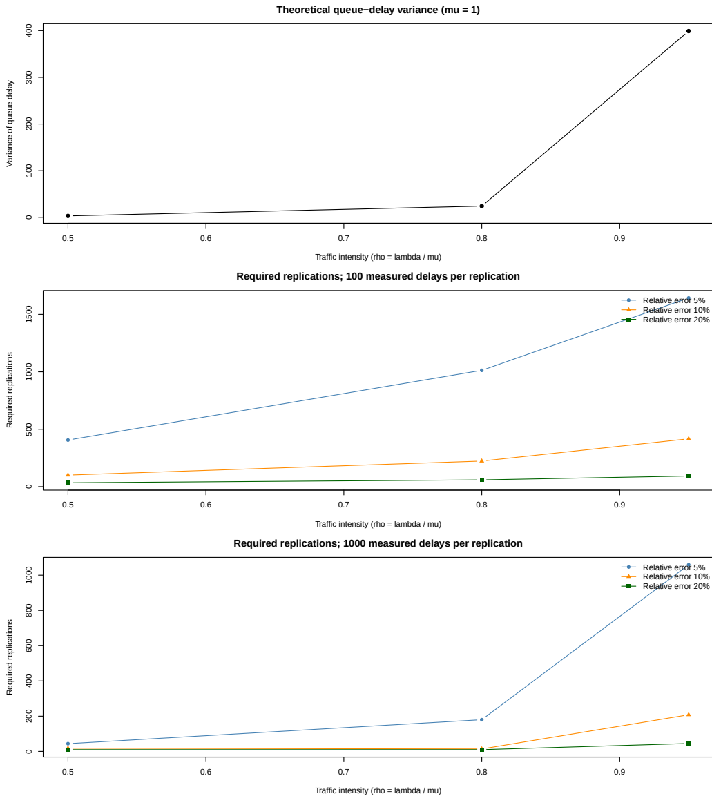
Figure 9: Theoretical queue-delay variance and observed replication requirements as functions of \rho , for two measured sample sizes.
