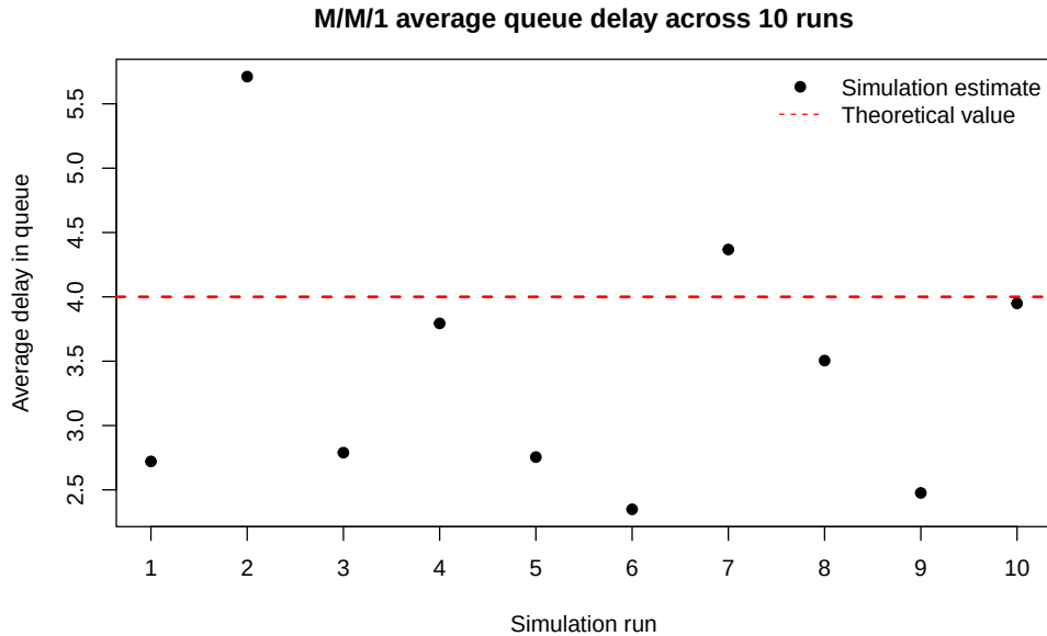
Figure 7: Average queue-delay estimate in each of the ten M/M/1 runs. The dashed line marks the theoretical value W_Q = 4 .
